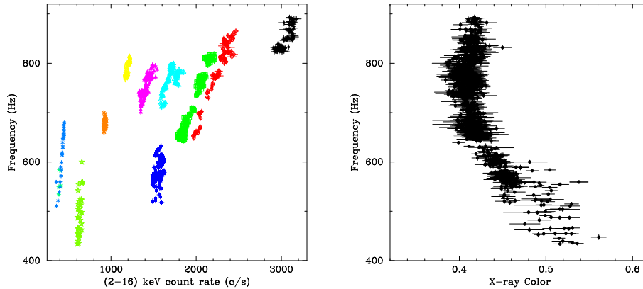
Figure 4. Left Panel: Relation between \nu_1 and the 2–16 keV count rate in 4U 1608–52. Right Panel: For the same data as on the left panel, \nu_1 vs. X-ray hard color, defined as the ratio of the count rate in the 6.0 – 9.7 keV band to the count rate in the 9.7 – 16.0 keV band.
